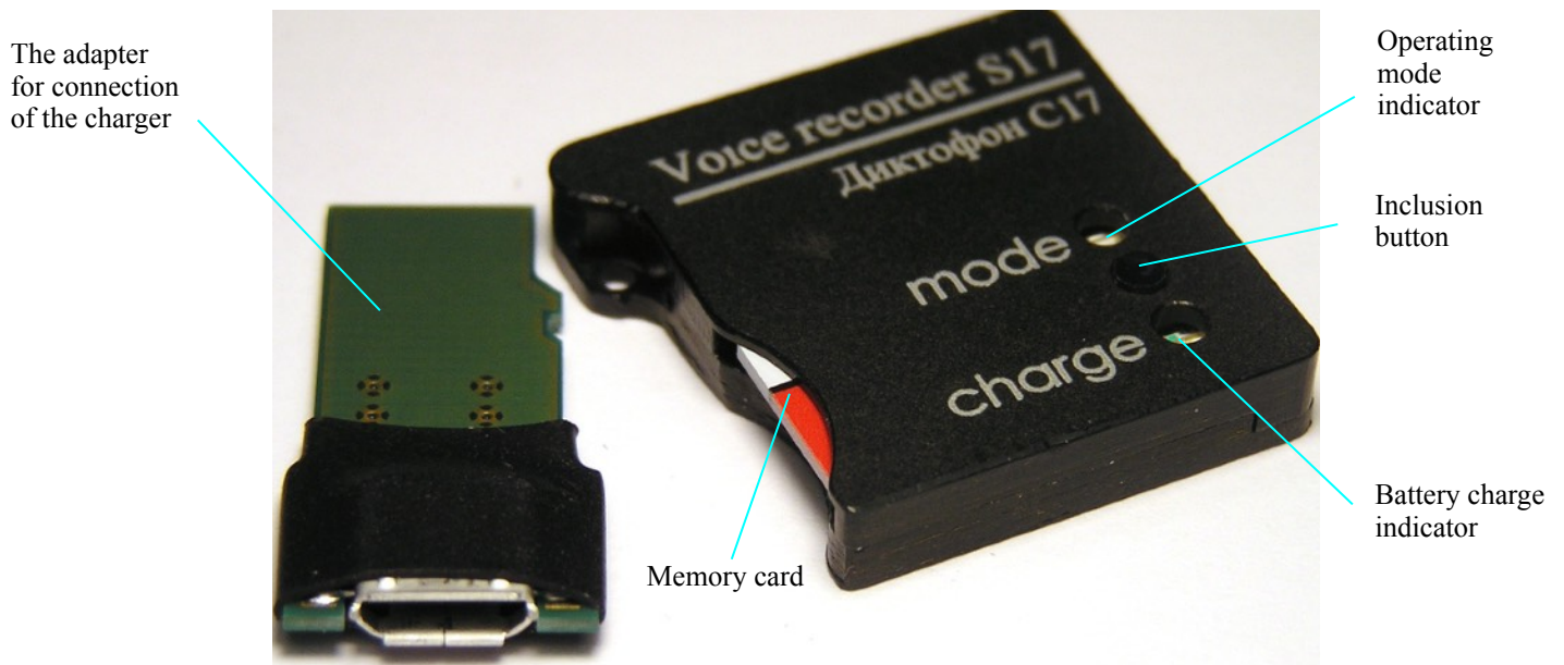
Fig. 2. Appearance of voice recorder Soroka-17E
